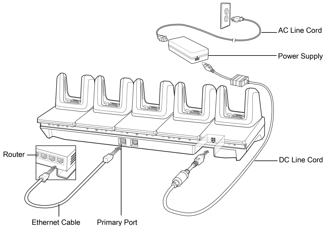
Figure 16 5-Slot Ethernet ShareCradle Setup
