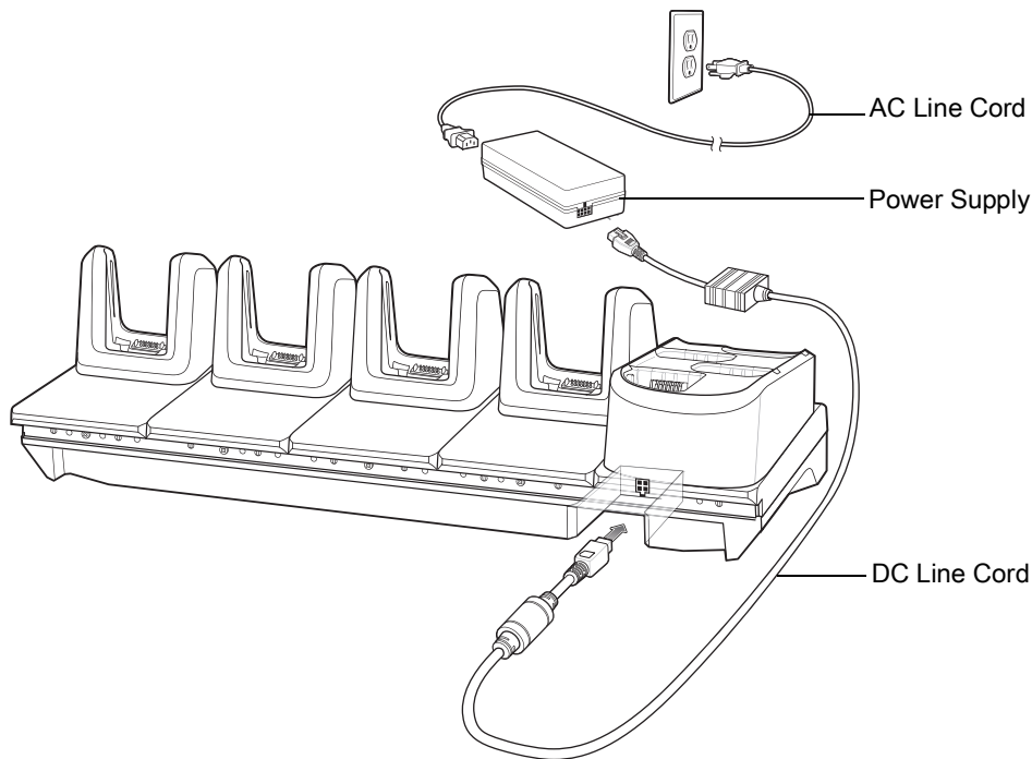
Figure 20 5-Slot ShareCradle with 4-Slot Battery Charger Setup
