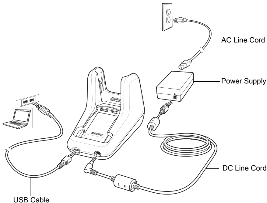
Figure 12 1-Slot USB Charge Cradle Setup
