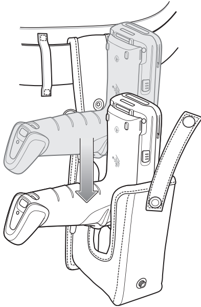
Figure 49 Insert MC33XX-G
