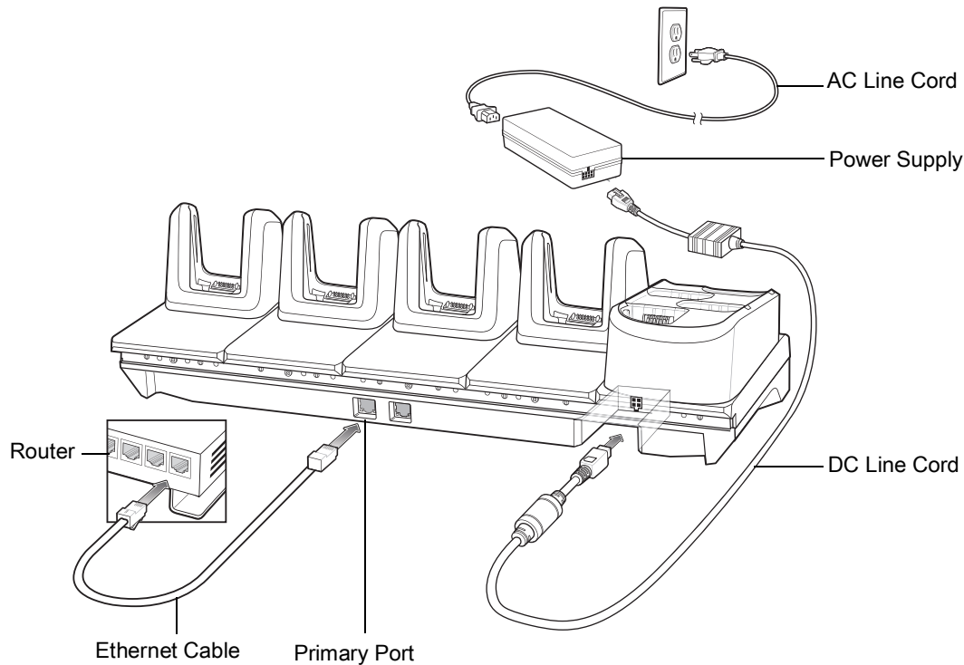
Figure 21 5-Slot Ethernet ShareCradle with 4-Slot Battery Charger Setup
