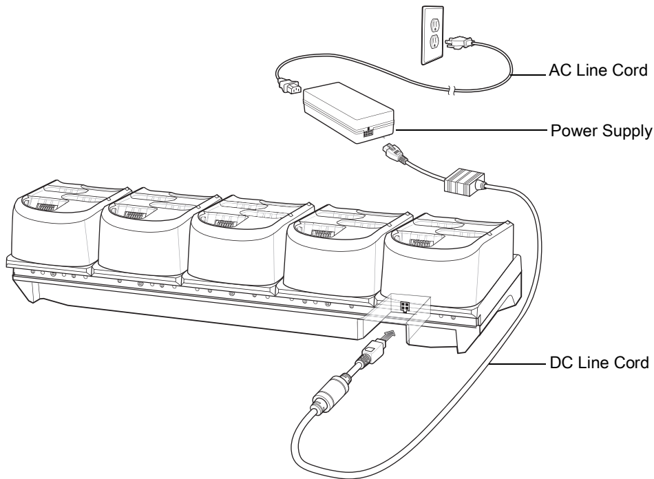
Figure 26 20-Slot Battery Charger Setup
