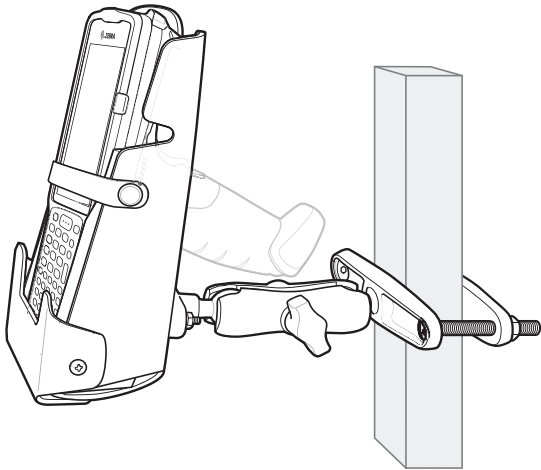
Figure 59 Forklift Mount
