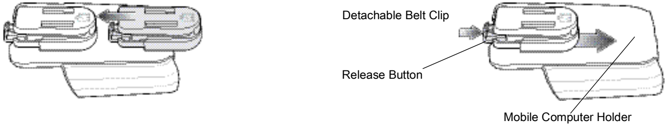
Figure 43 Plastic Holster
