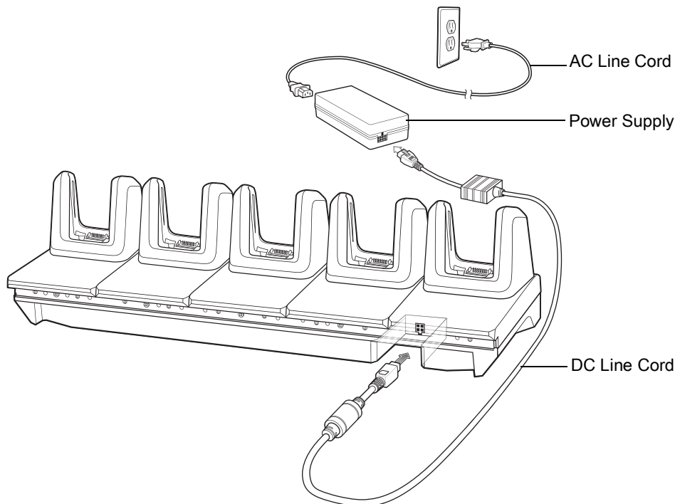
Figure 15 5-Slot Charge Only ShareCradle Setup
