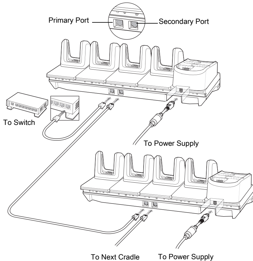
Figure 22 Daisy-chaining 5-Slot Ethernet ShareCradle with 4-Slot Battery Chargers
