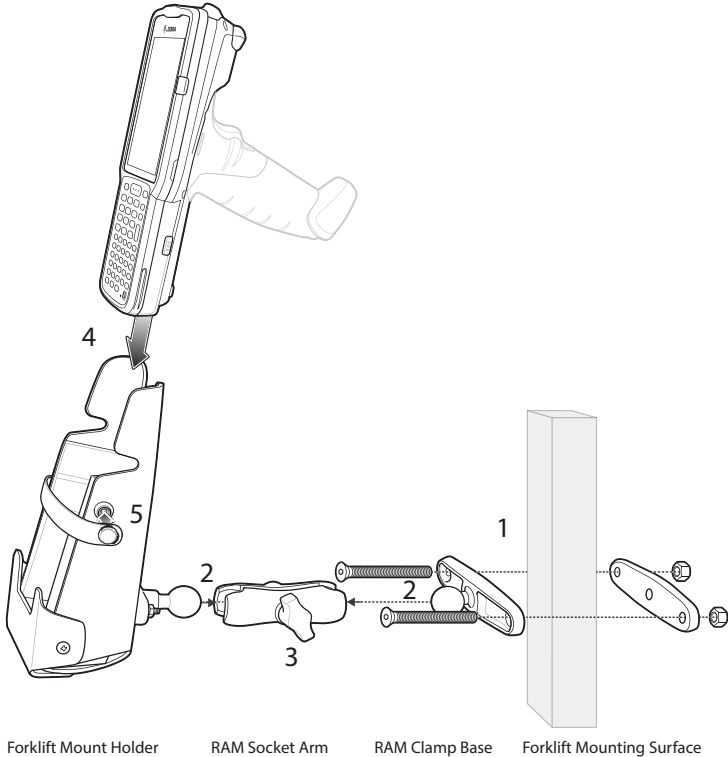
Figure 60 Forklift Mount Assembly
