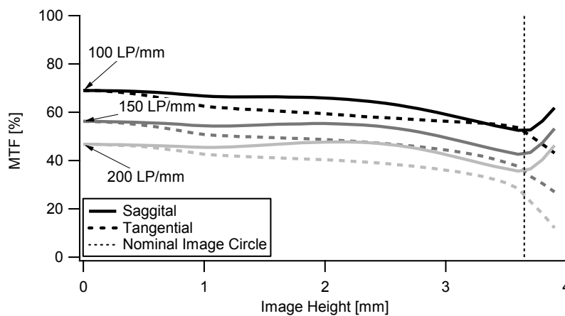
Figure 6: Resolution vs. Image Height
